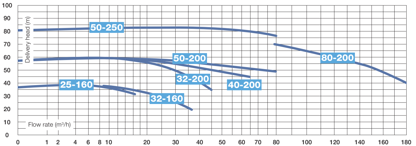
Characteristic curves NM (n = 2900 rpm, 50 Hz)
